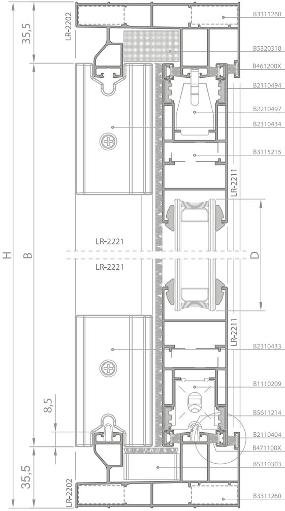
17-17 Detay 17-17 Details
