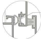
Alternatif Detay Alternative Details
