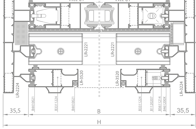
55-55 Detay 55-55 Details
