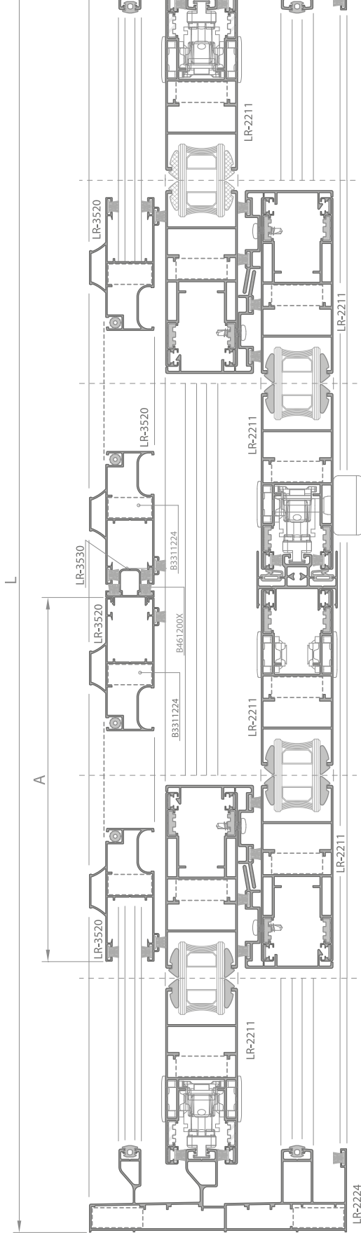
54-54 Detay 54-54 Details
