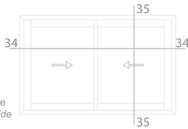
Alternatif Detay Alternative Details
