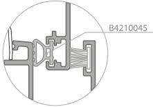
Alternatif Detay-2 Alternative Details-2
