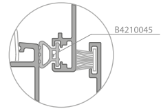
Alternatif Detay-2 Alternative Details-2
