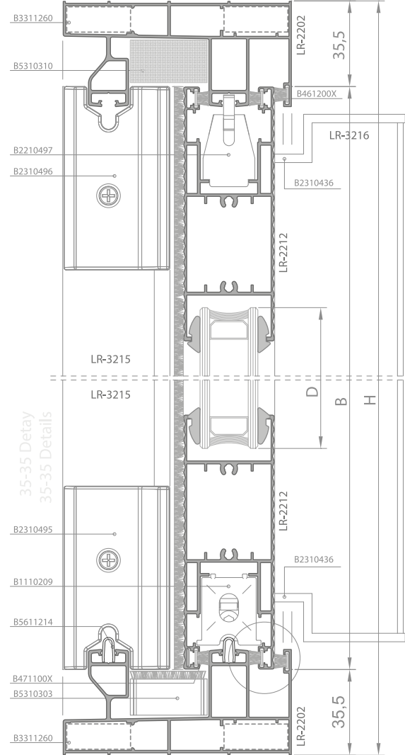
34-34 Detay 34-34 Details
