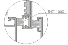
Alternatif Detay-1 Alternative Details-1
