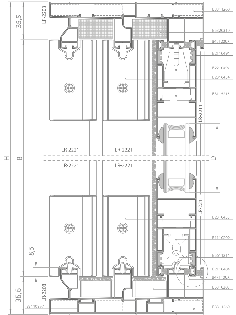
14-14 Detay 14-14 Details
